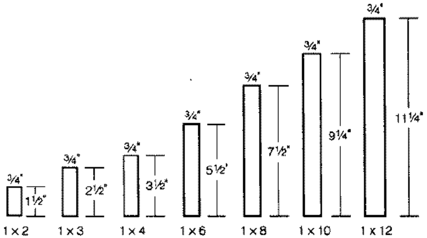
Approximate dimensions of stock lumber 1" thick
