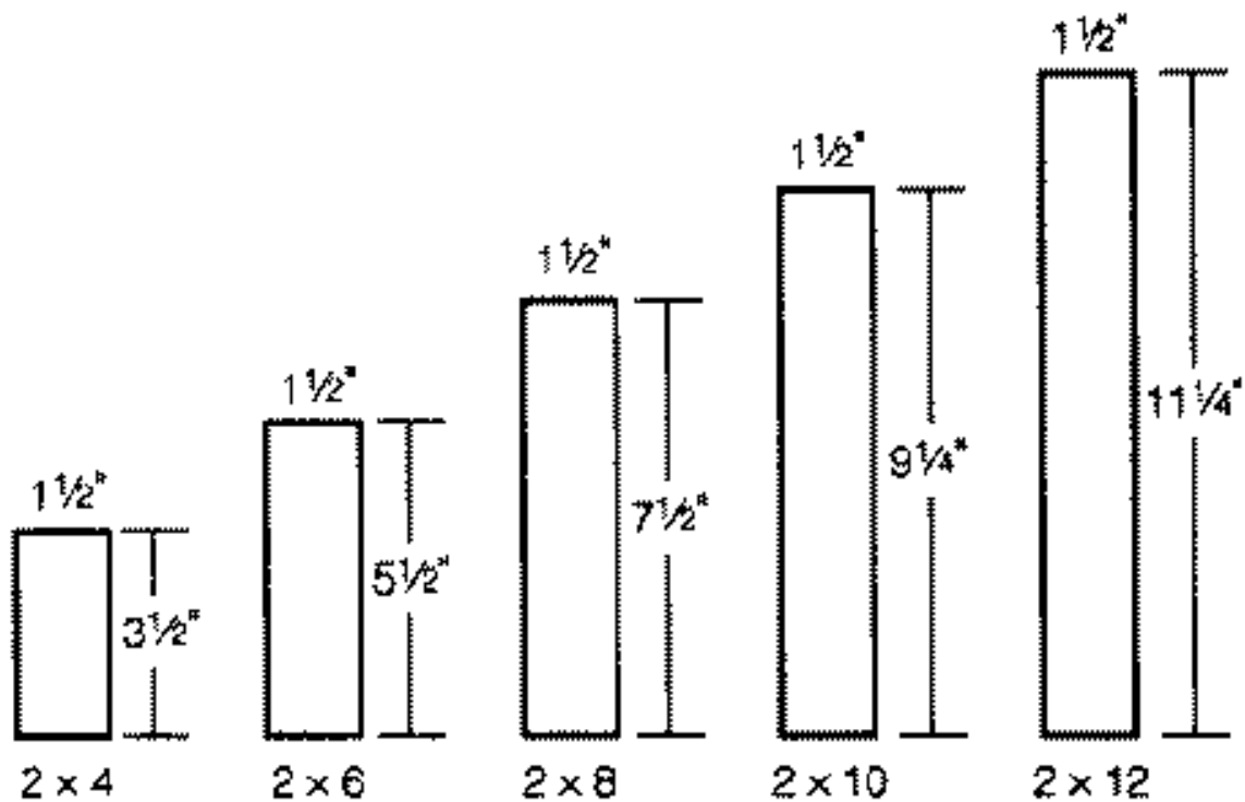
Approximate dimensions of 2" thick stock lumber
